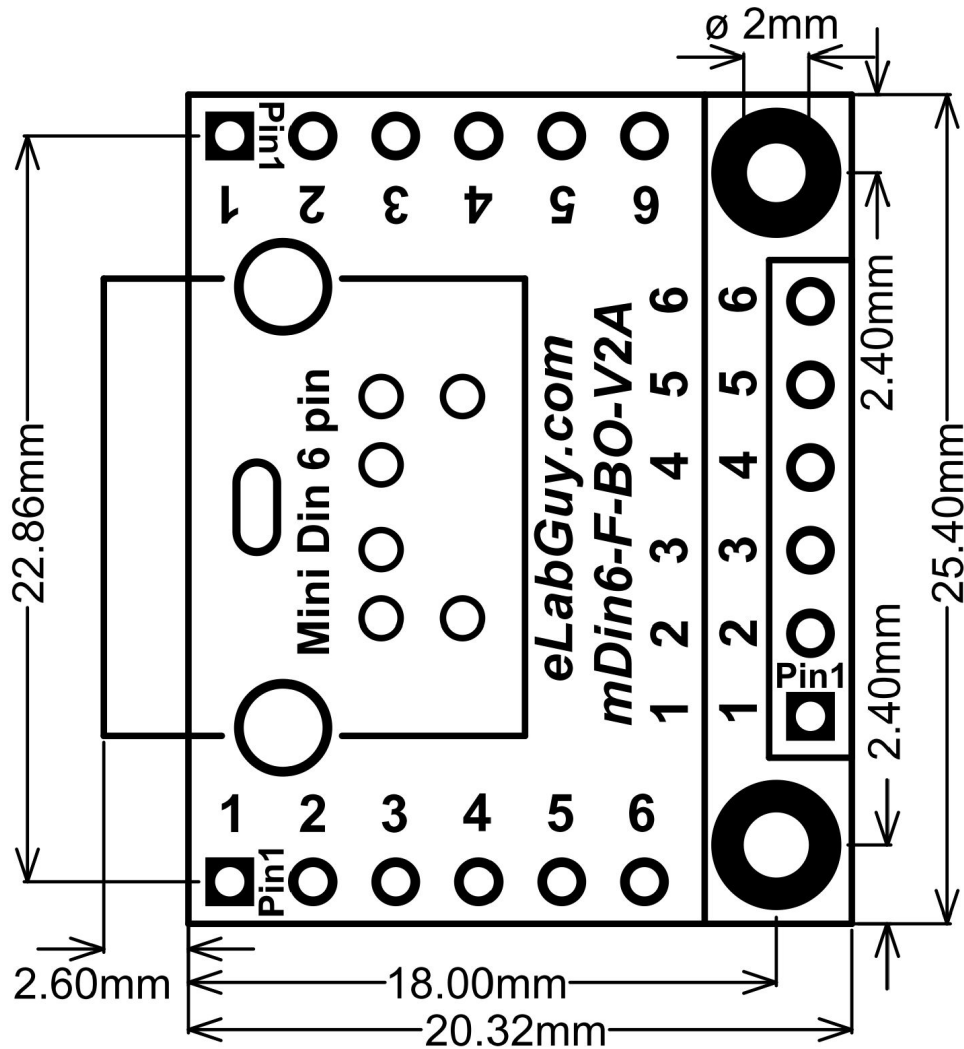
mDin6-F-BO-V1A PCB outline Drawing
